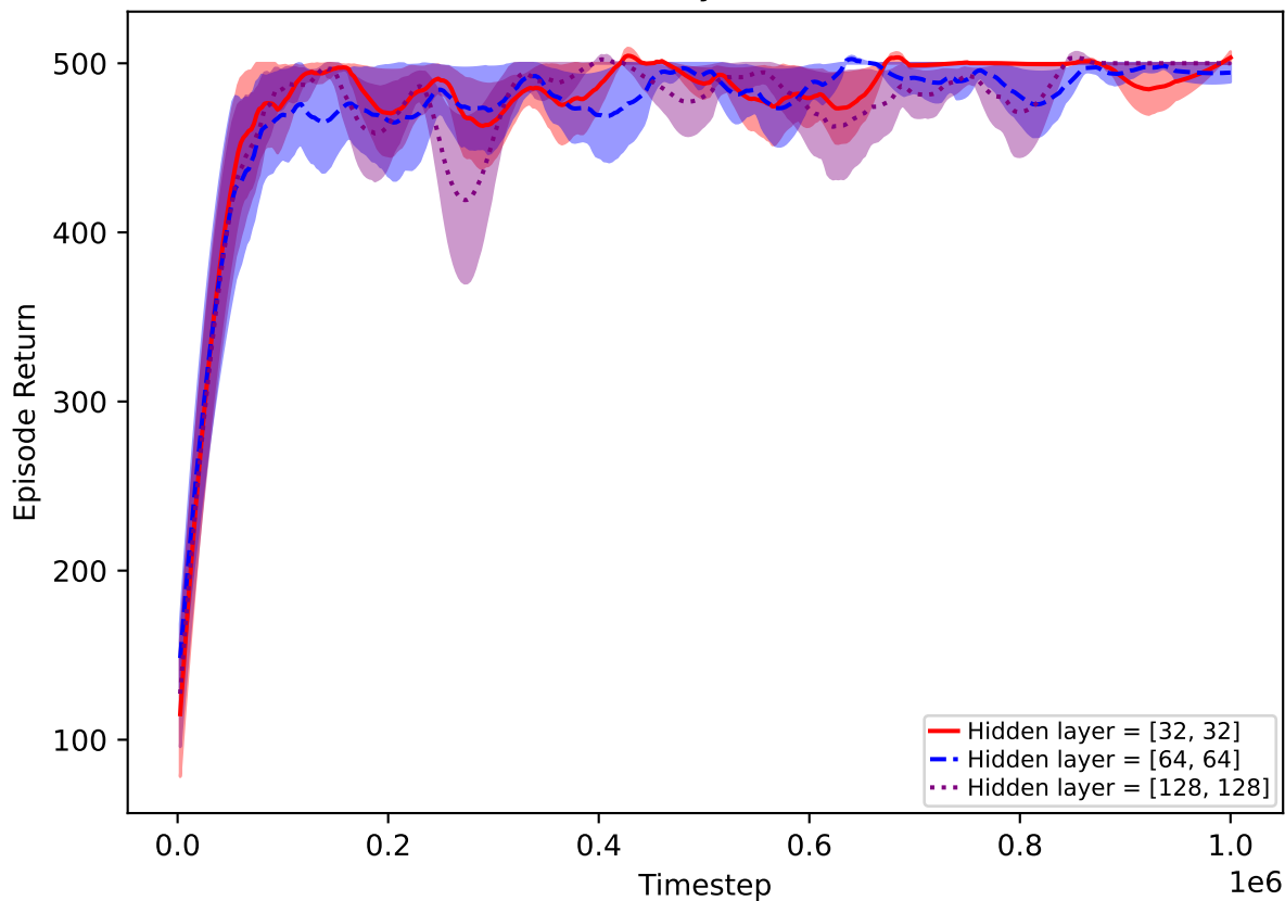
Critic hidden layer architecture
